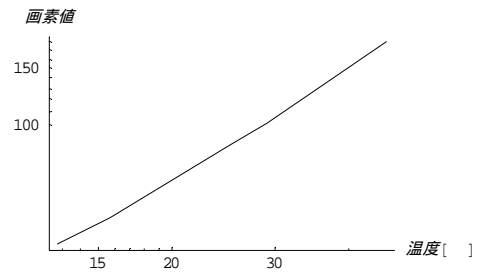
Fig. 2 Temperature versus pixel value relation
