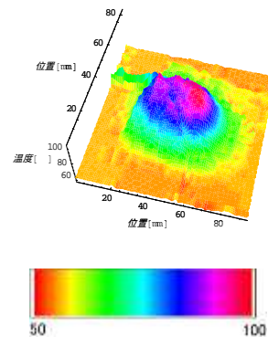
Fig.4 Absolute Temperature Distribution of the Iron Sheet shown in Fig.3
