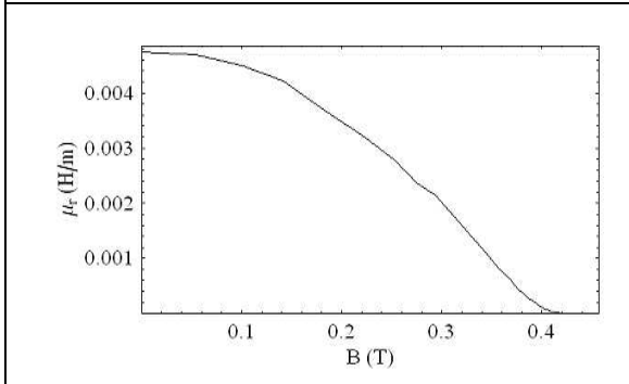
Fig.2 Reversible Permeability \mu_r (TDK H5A)
