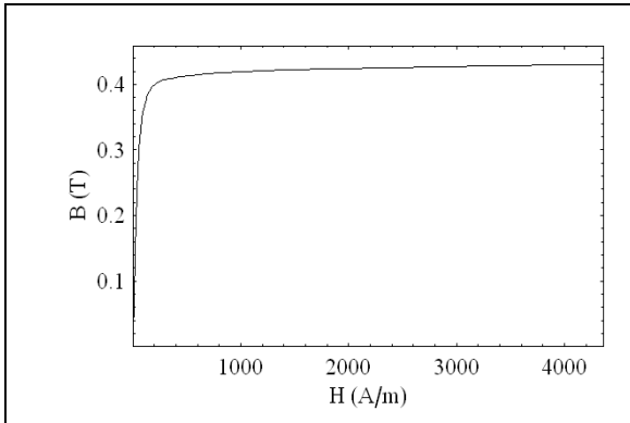
Fig.1 Magnetization Curve Giving Permeability \mu (TDK H5A)
