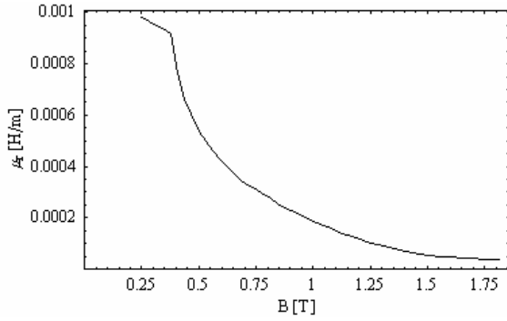
Fig. 2. Reversible permeability \mu_r (soft iron)
