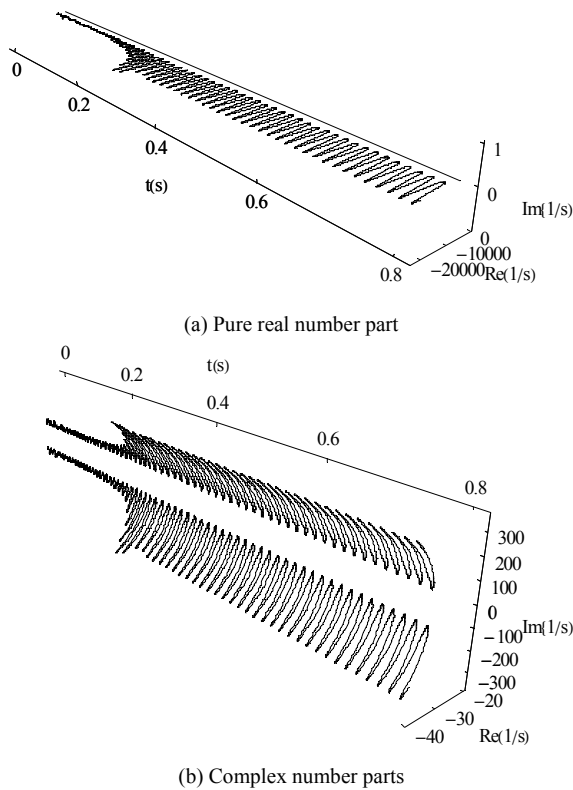
Fig.8. Changes of the characteristic values derived from the state transition matrix a in Eq.(8)
