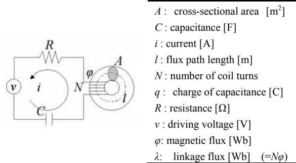
Fig. 4. Series ferroresonant circuit
