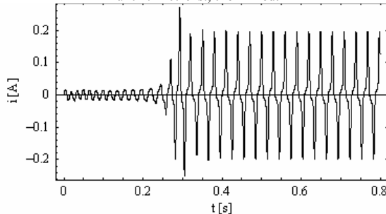
Fig. 6. Calculated current i vs. time t
