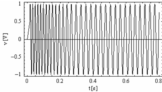
Fig. 5. Driving voltage. Frequency is decreased from 70 to 33 Hz until t = 0.29 s., then fixed.
