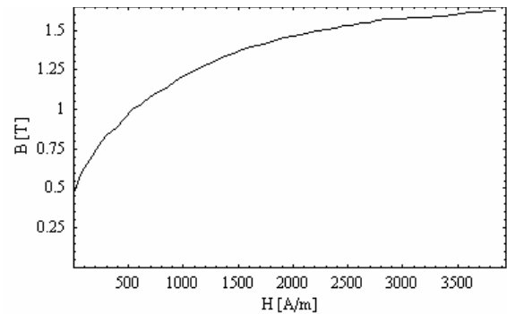
Fig. 1. Magnetization curve giving permeability \mu (soft iron)
