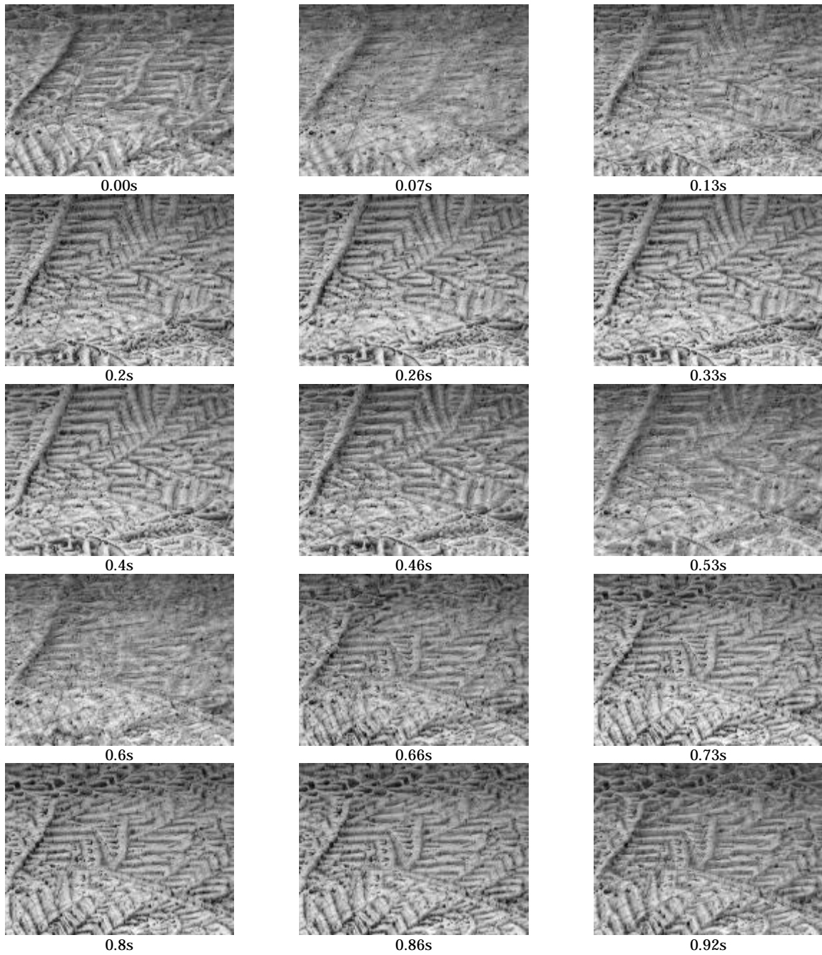
Fig.2 Visualized Magnetic Domain Images by Bitter Method
