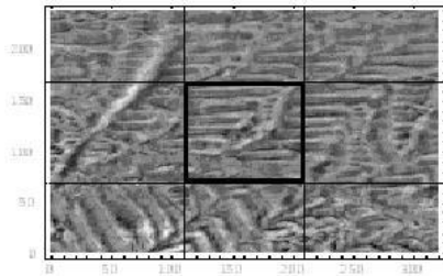
Fig.6 Sample Area for Local Magnetization Characteristic Extraction
