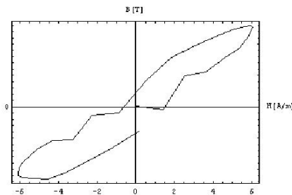
Fig.7 Local Magnetization Characteristic Curve in the Area enclosed by Black Square Box
