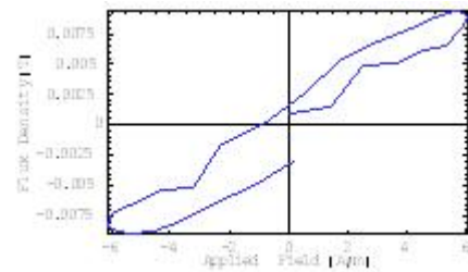
Fig.5 Averaged Magnetization Characteristic Curve
