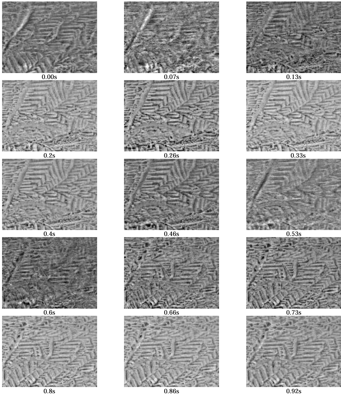
Fig.4 Dynamic Magnetic Domain Images not Including Static Background Image in Fig. 3
