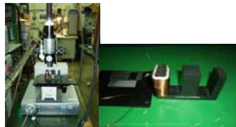
Fig.1 Tested Yoke and Exciting Coil
