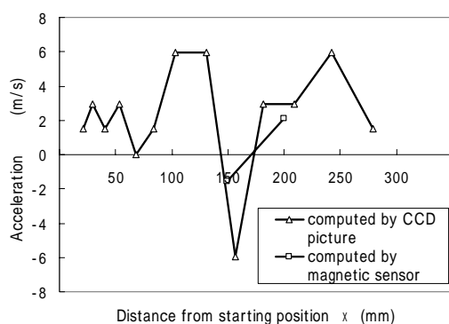
Fig.10 Evaluated Acceleration.
