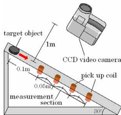
Fig.4 Schematic Diagram of the Tested Sloping Transport System.
